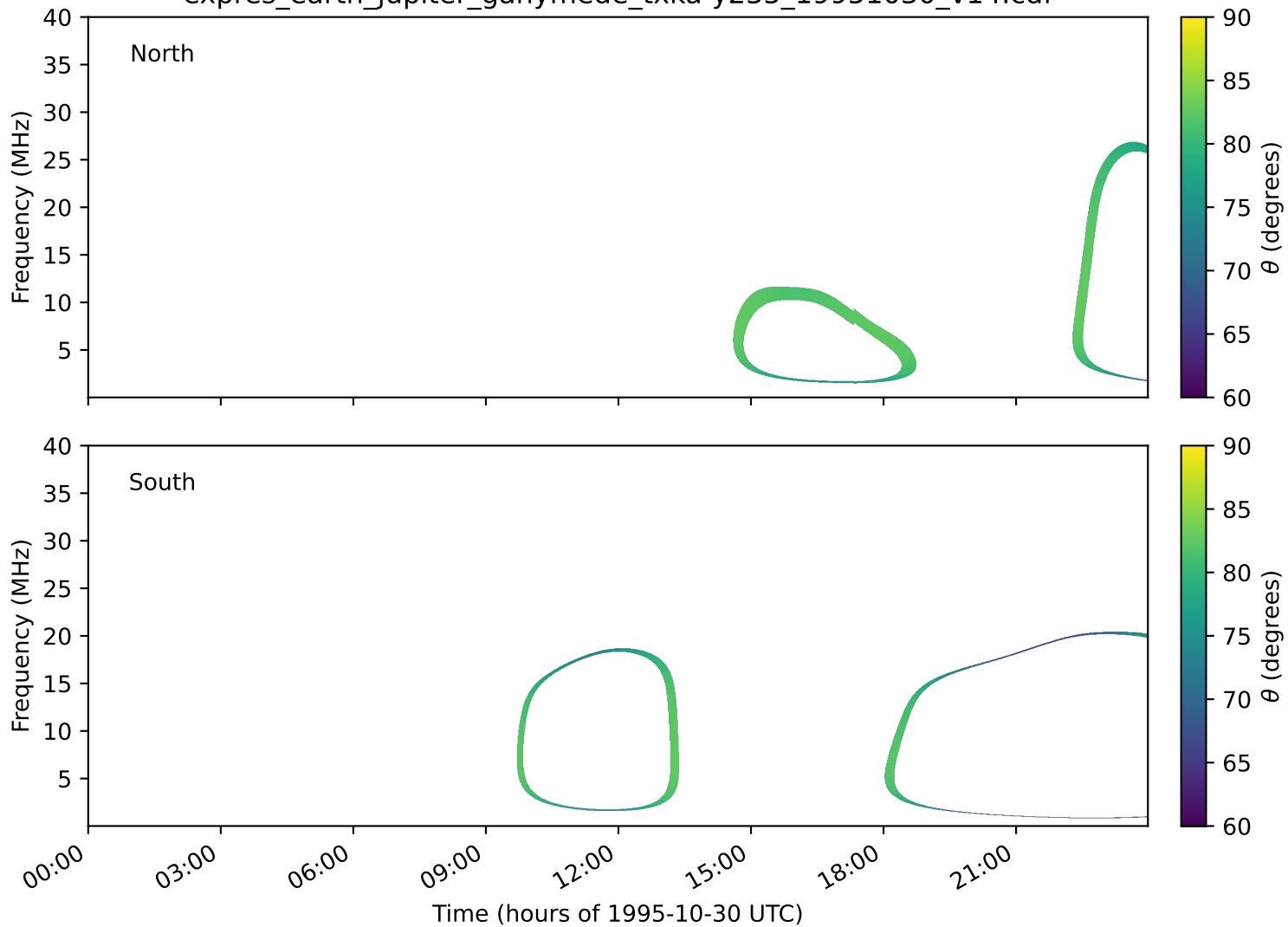
expres_earth_jupiter_ganymede_txka-y235_19951030_v14.cdf
