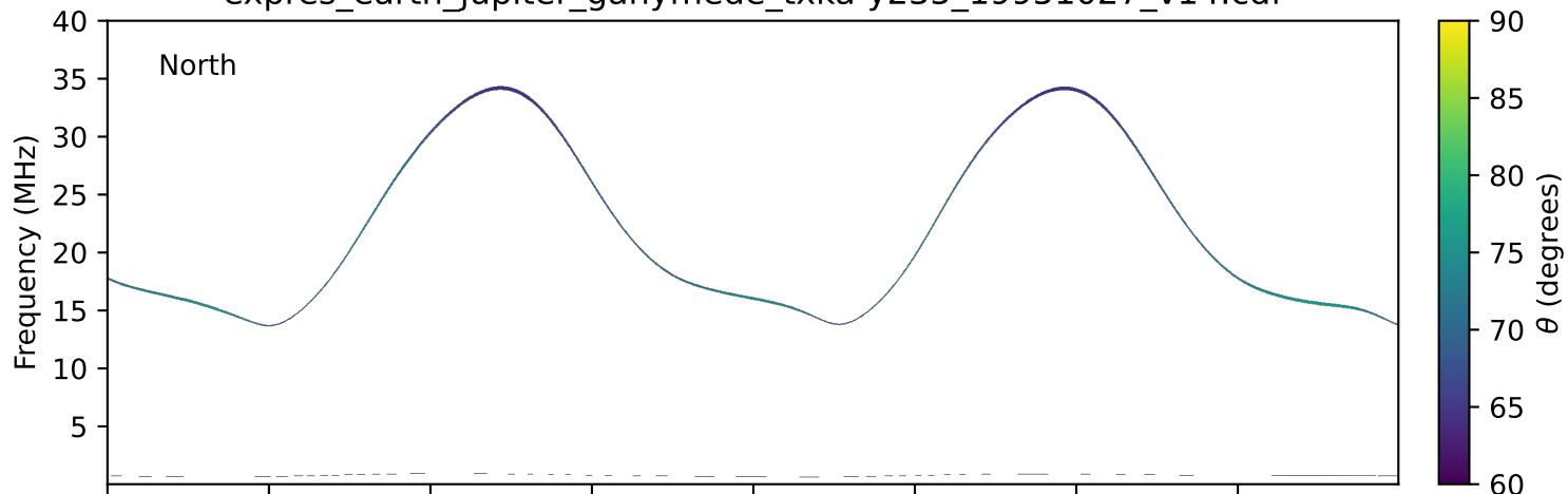
expres_earth_jupiter_ganymede_txka-y235_19951027_v14.cdf
