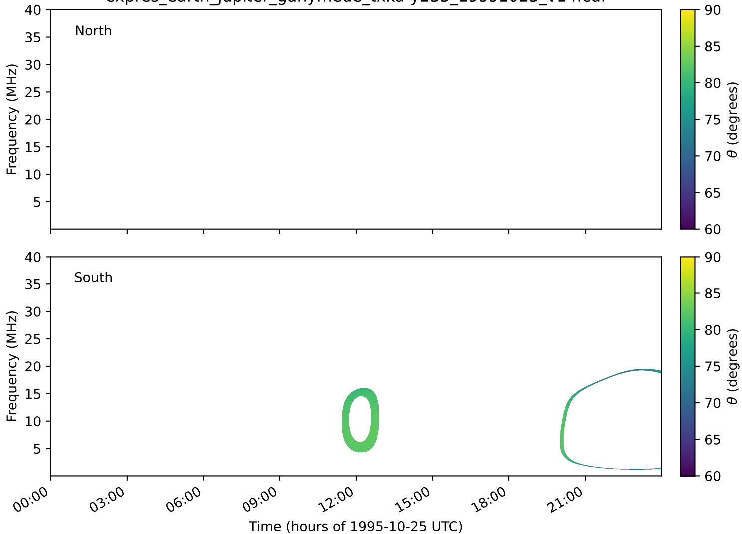
expres_earth_jupiter_ganymede_txka-y235_19951025_v14.cdf
