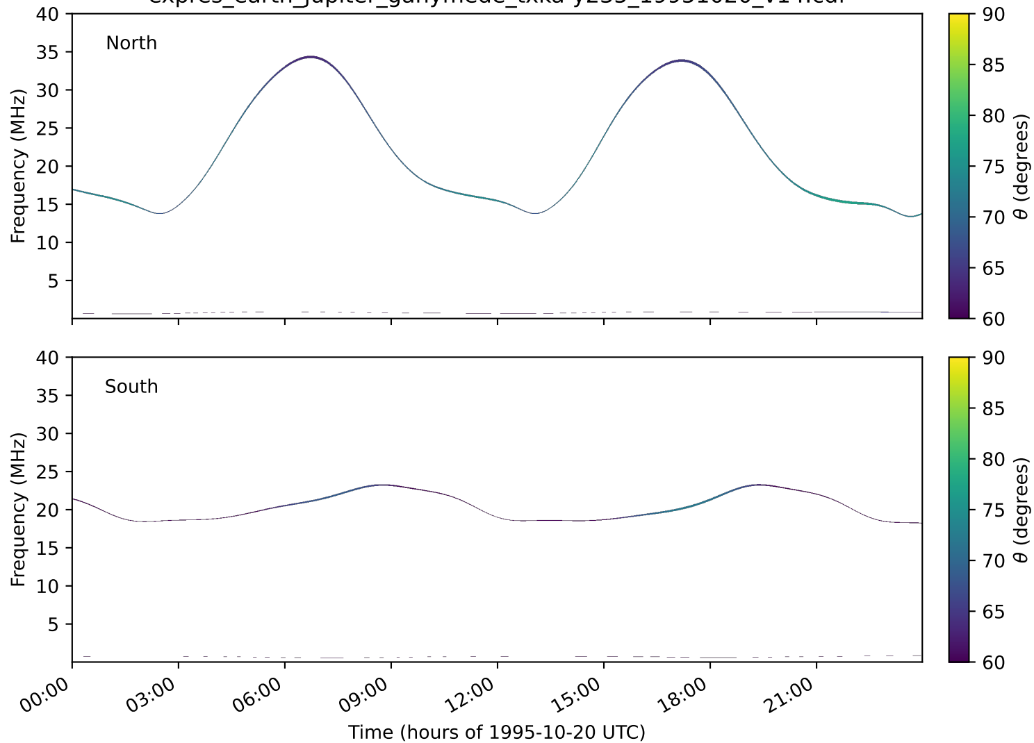
expres_earth_jupiter_ganymede_txka-y235_19951020_v14.cdf
