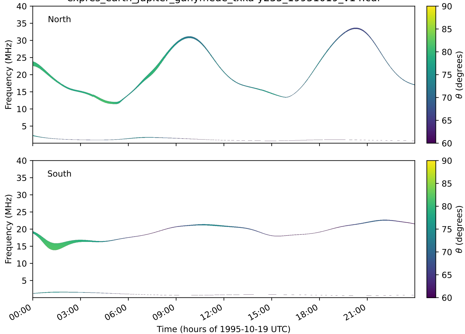
expres_earth_jupiter_ganymede_txka-y235_19951019_v14.cdf
