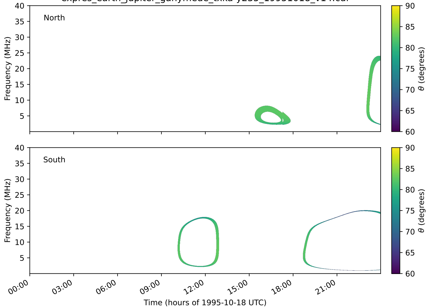
expres_earth_jupiter_ganymede_txka-y235_19951018_v14.cdf
