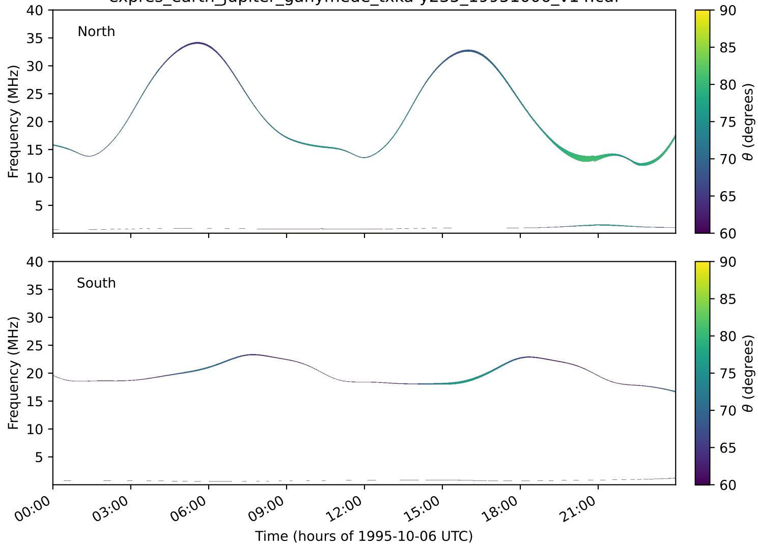
expres_earth_jupiter_ganymede_txka-y235_19951006_v14.cdf
