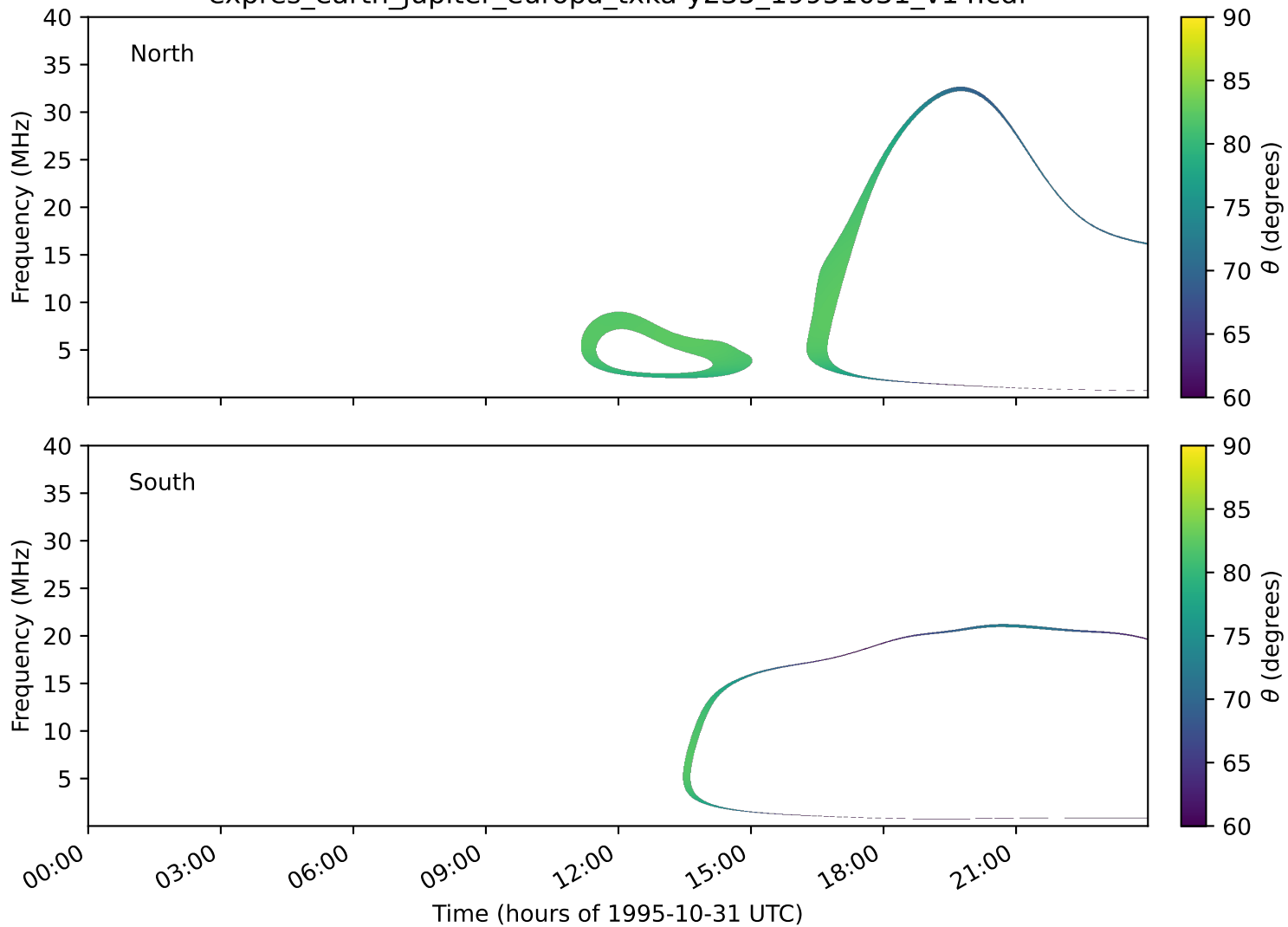
expres_earth_jupiter_europa_txka-y235_19951031_v14.cdf
