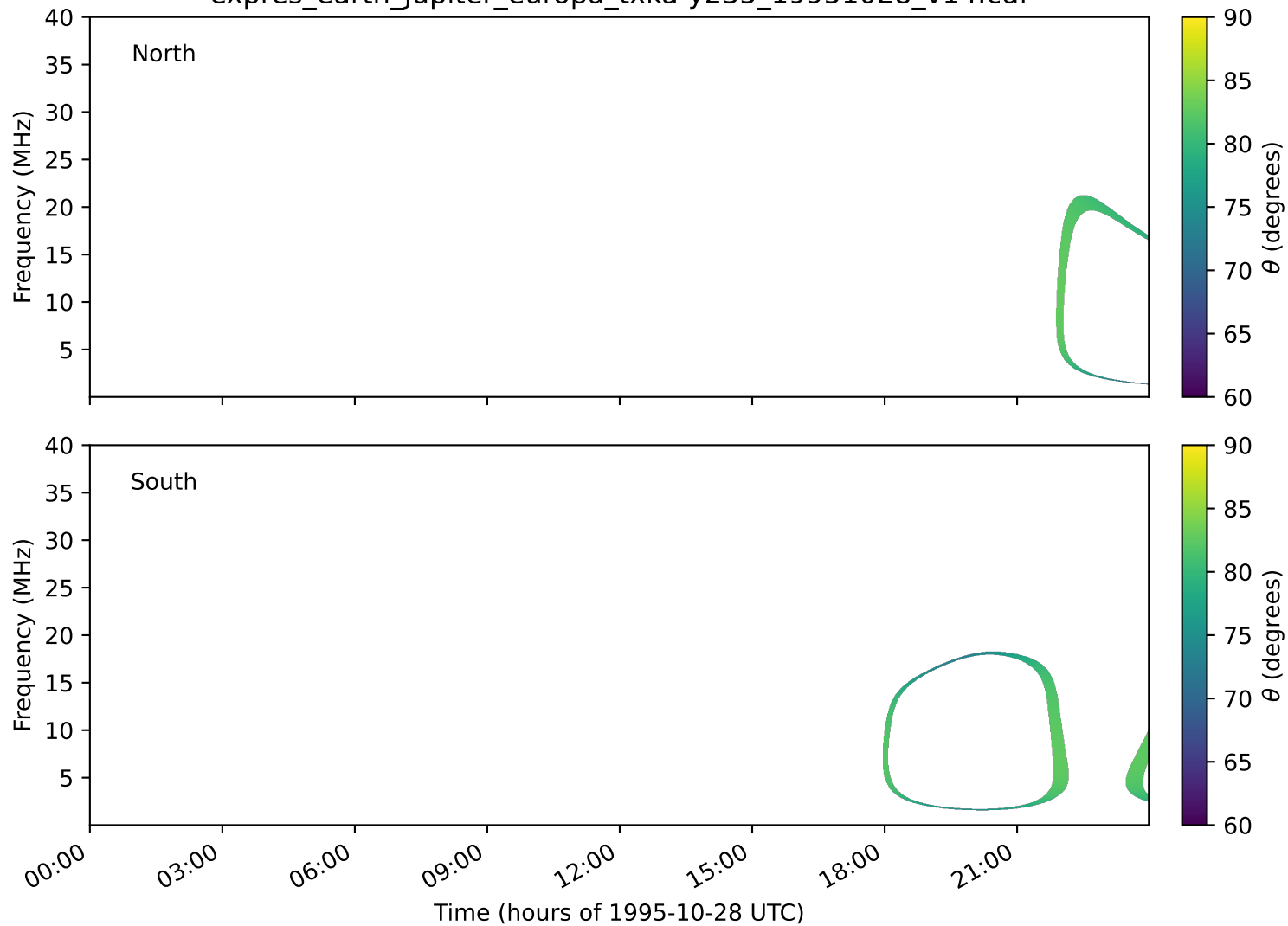
expres_earth_jupiter_europa_txka-y235_19951028_v14.cdf
