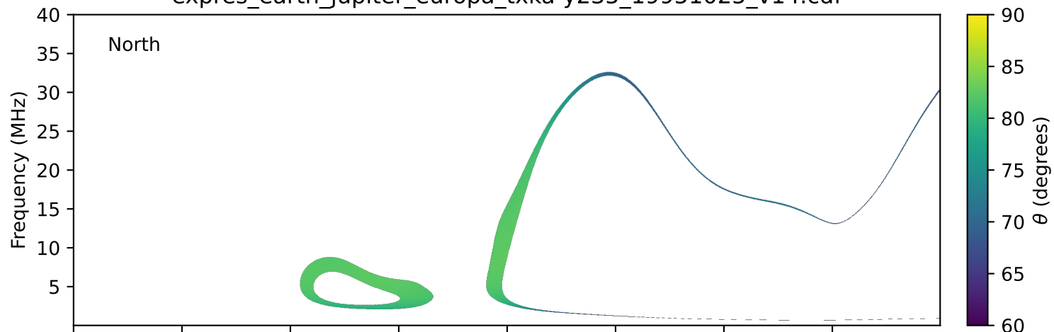
expres_earth_jupiter_europa_txka-y235_19951025_v14.cdf
