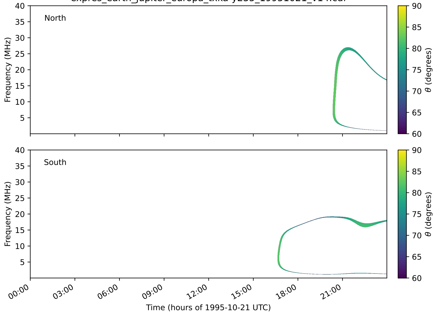
expres_earth_jupiter_europa_txka-y235_19951021_v14.cdf
