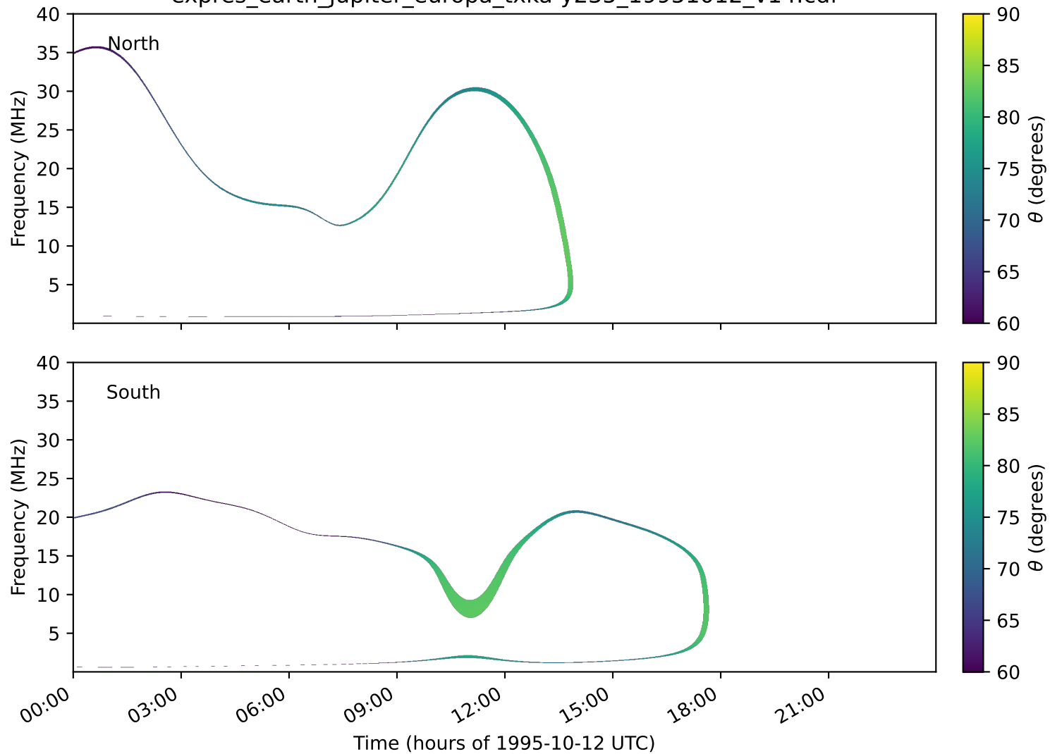
expres_earth_jupiter_europa_txka-y235_19951012_v14.cdf
