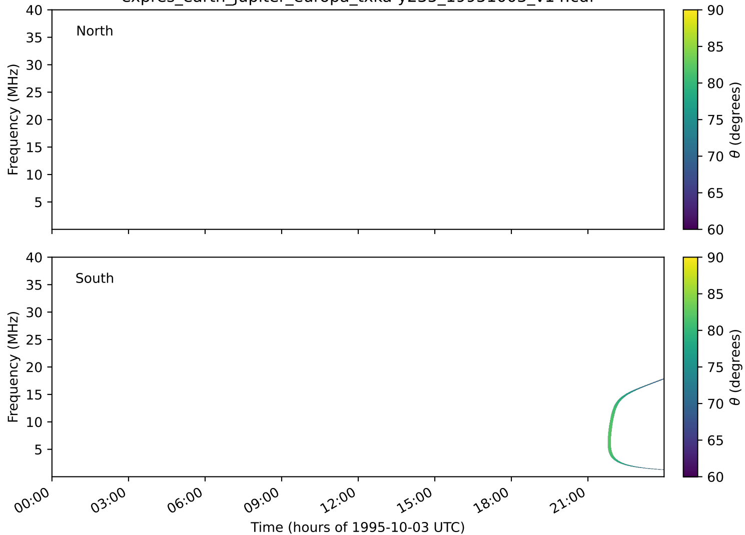
expres_earth_jupiter_europa_txka-y235_19951003_v14.cdf
