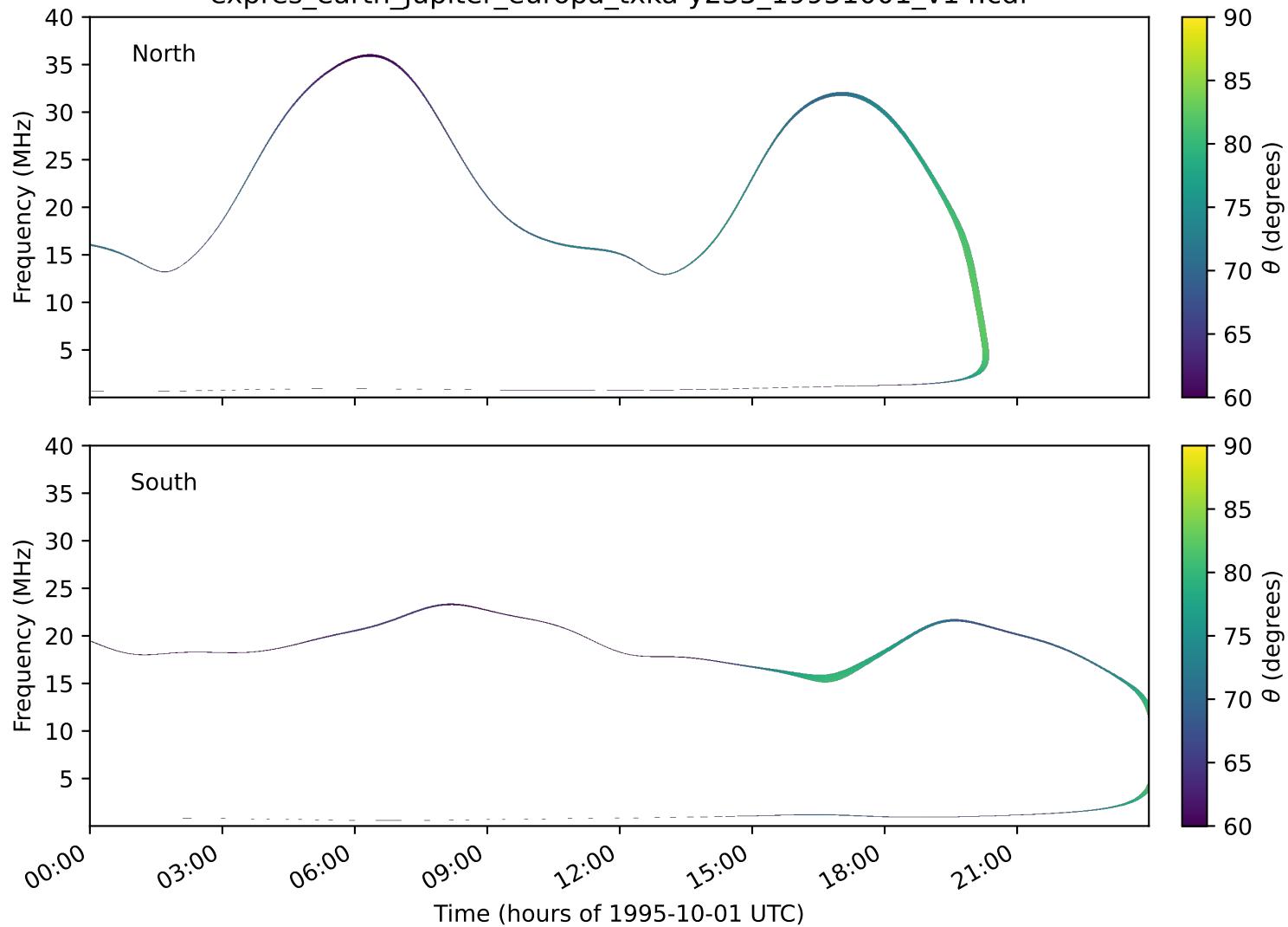
expres_earth_jupiter_europa_txka-y235_19951001_v14.cdf
