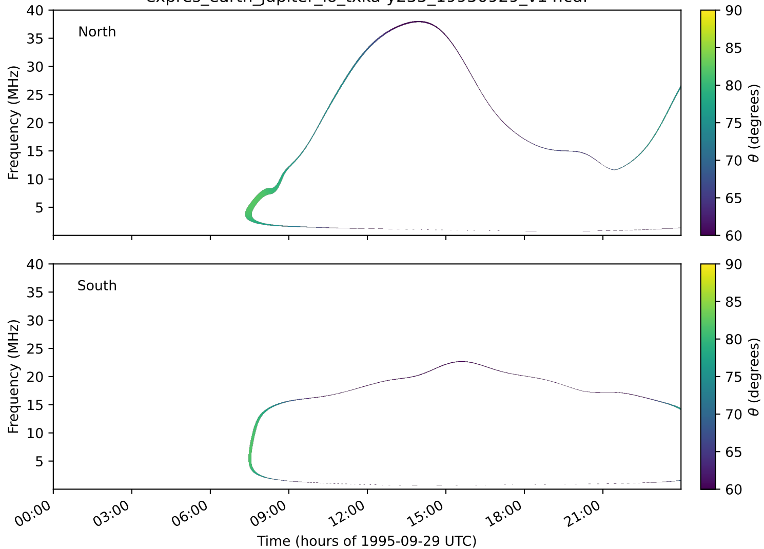
expres_earth_jupiter_io_txka-y235_19950929_v14.cdf
