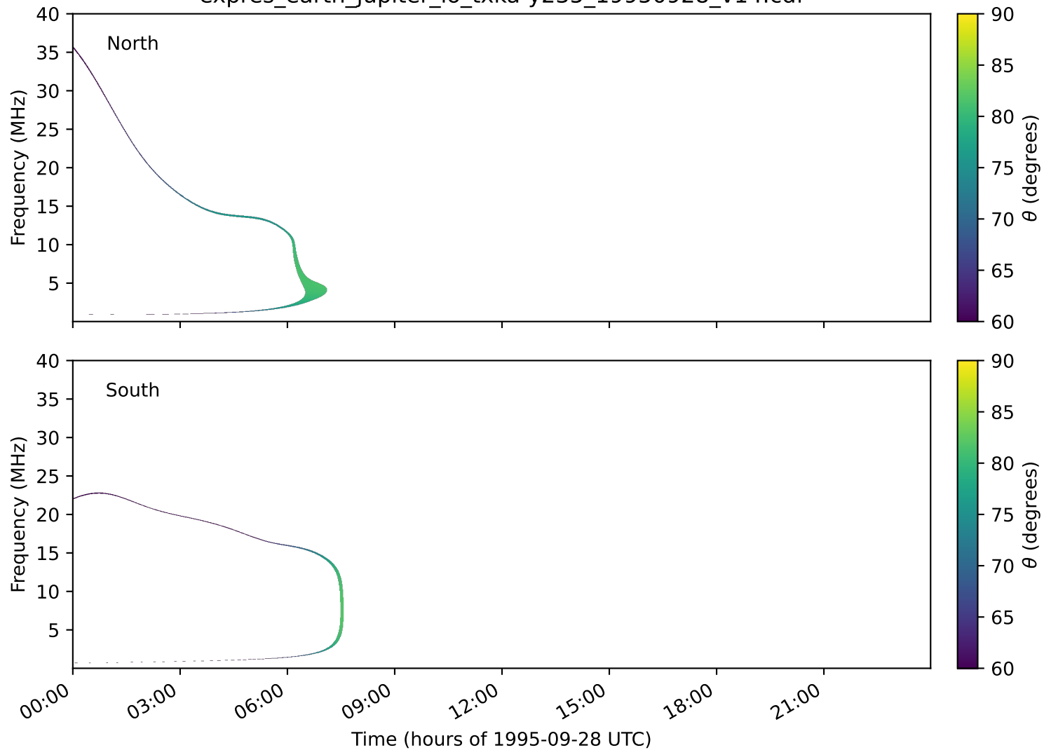
expres_earth_jupiter_io_txka-y235_19950928_v14.cdf
