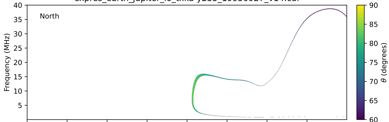
expres_earth_jupiter_io_txka-y235_19950927_v14.cdf
