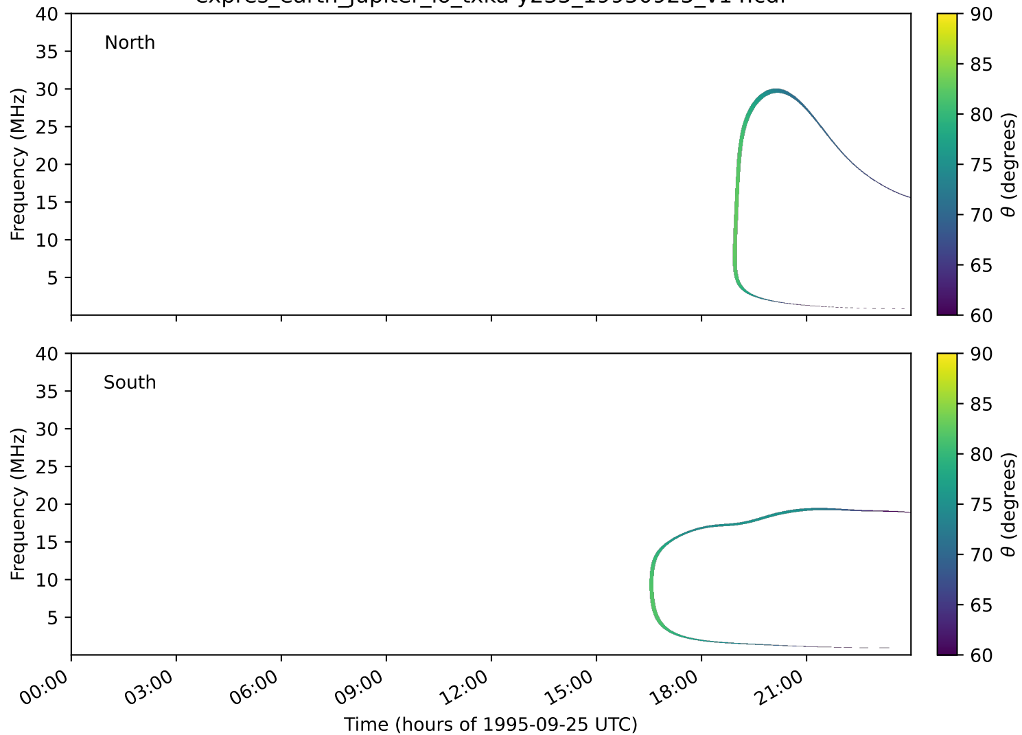
expres_earth_jupiter_io_txka-y235_19950925_v14.cdf
