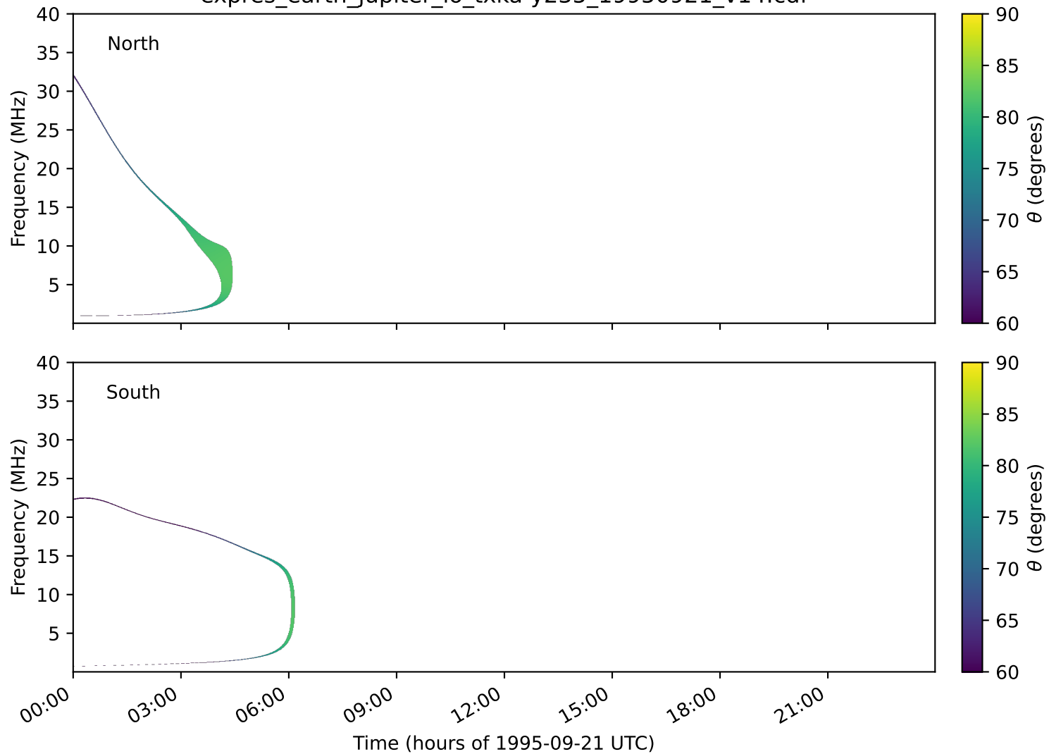
expres_earth_jupiter_io_txka-y235_19950921_v14.cdf
