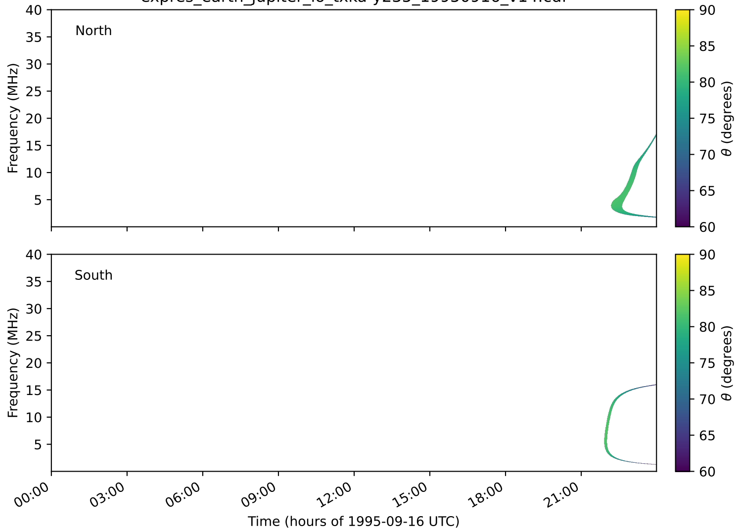
expres_earth_jupiter_io_txka-y235_19950916_v14.cdf
