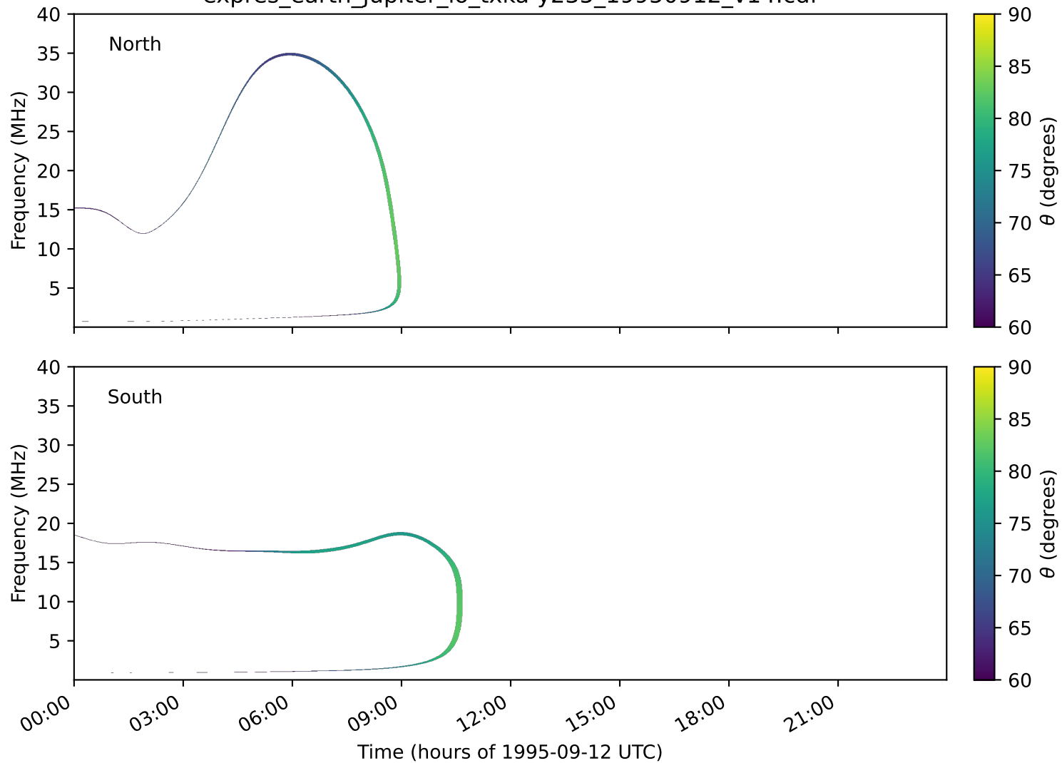
expres_earth_jupiter_io_txka-y235_19950912_v14.cdf
