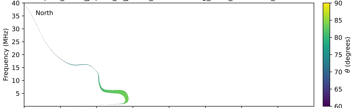
expres_earth_jupiter_io_jrm33_lossc-wid1deg_3kev_19950928_v11.cdf
