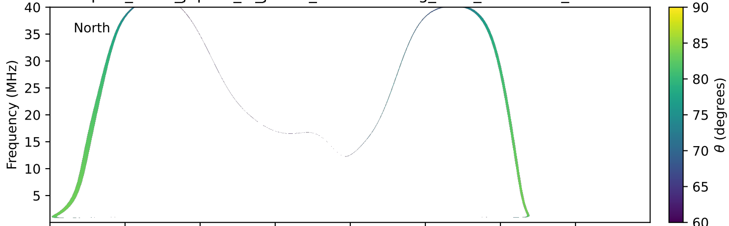
expres_earth_jupiter_io_jrm33_lossc-wid1deg_3kev_19950924_v11.cdf
