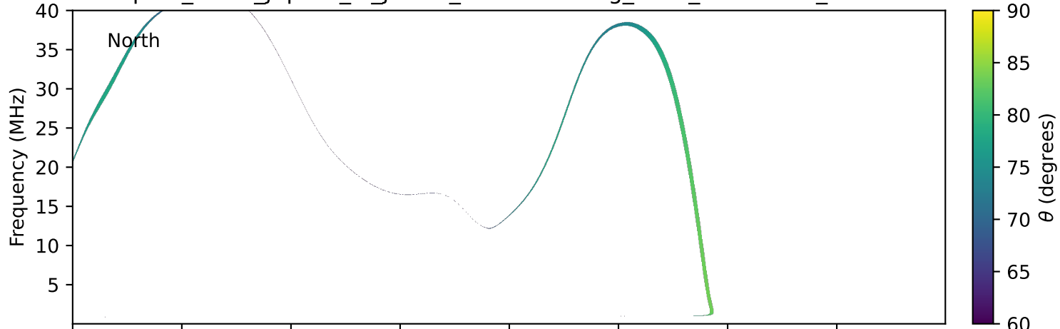
expres_earth_jupiter_io_jrm33_lossc-wid1deg_3kev_19950917_v11.cdf
