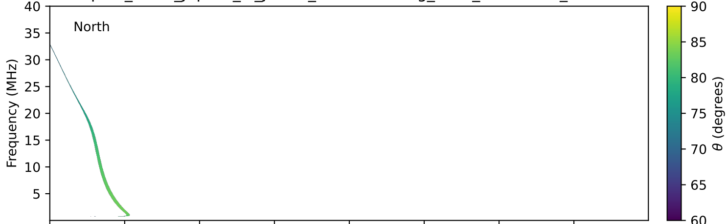
expres_earth_jupiter_io_jrm33_lossc-wid1deg_3kev_19950914_v11.cdf
