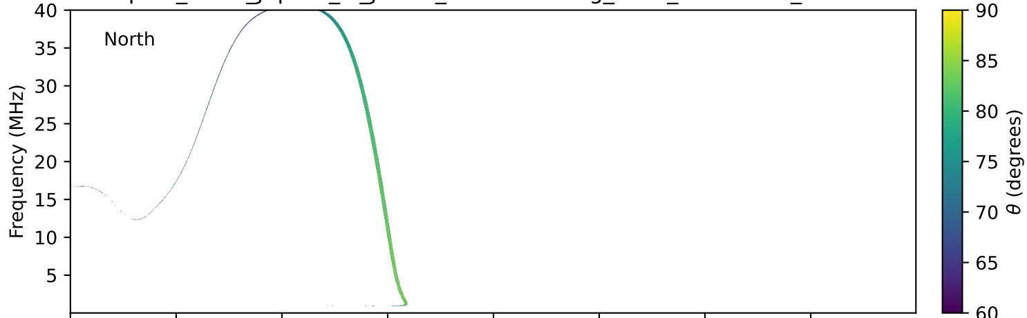
expres_earth_jupiter_io_jrm33_lossc-wid1deg_3kev_19950912_v11.cdf
