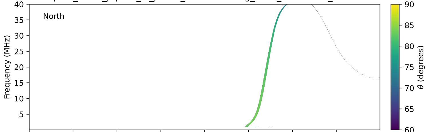
expres_earth_jupiter_io_jrm33_lossc-wid1deg_3kev_19950911_v11.cdf
