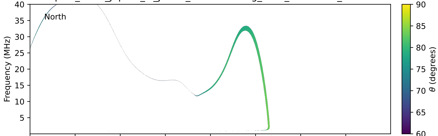
expres_earth_jupiter_io_jrm33_lossc-wid1deg_3kev_19950910_v11.cdf
