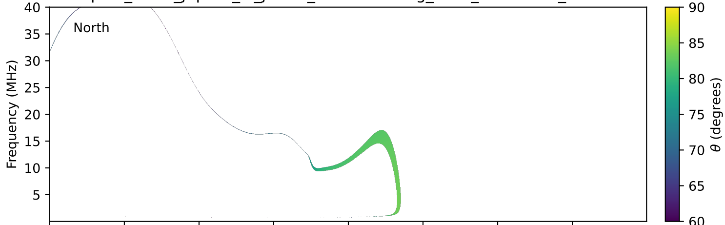
expres_earth_jupiter_io_jrm33_lossc-wid1deg_3kev_19950903_v11.cdf
