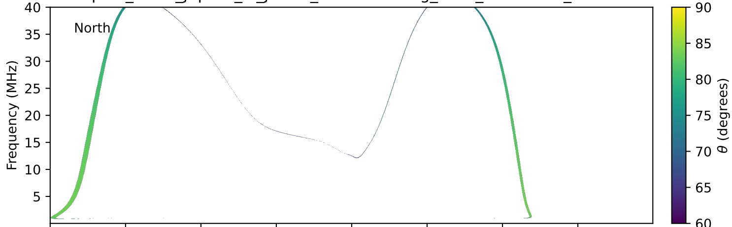
expres_earth_jupiter_io_jrm09_lossc-wid1deg_3kev_19950924_v11.cdf
