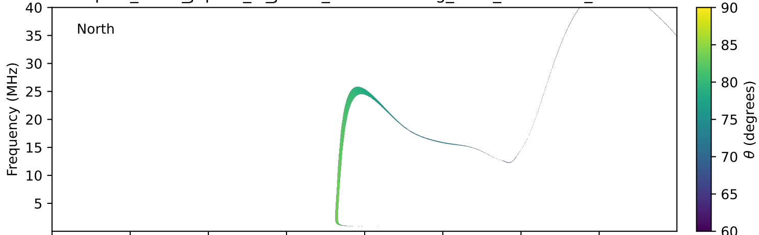
expres_earth_jupiter_io_jrm09_lossc-wid1deg_3kev_19950920_v11.cdf
