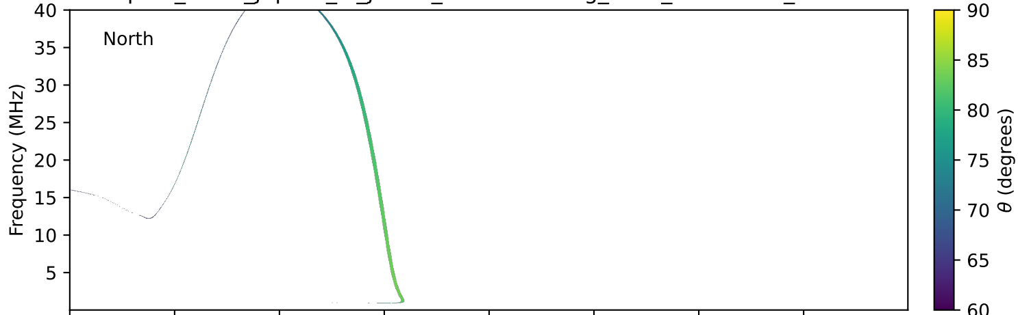
expres_earth_jupiter_io_jrm09_lossc-wid1deg_3kev_19950912_v11.cdf
