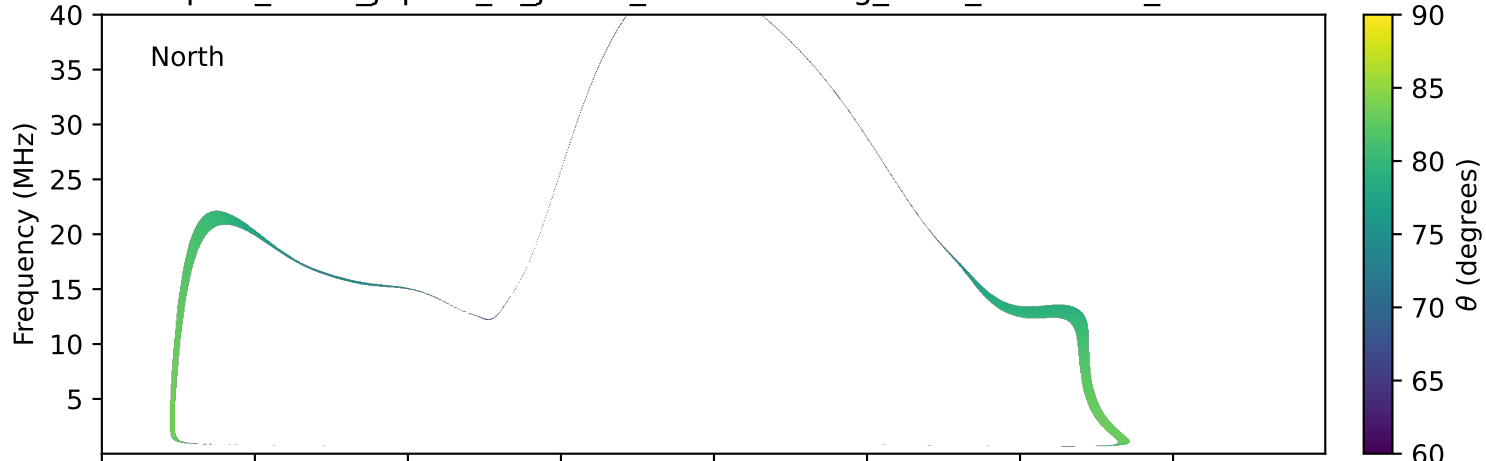
expres_earth_jupiter_io_jrm09_lossc-wid1deg_3kev_19950908_v11.cdf
