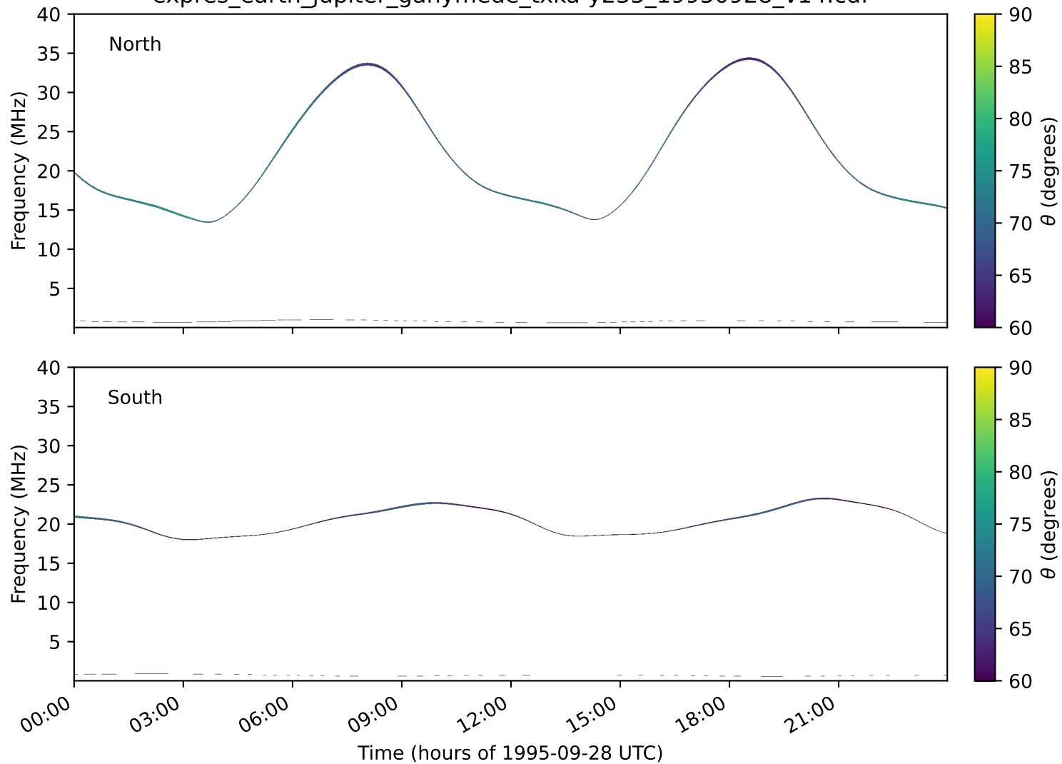
expres_earth_jupiter_ganymede_txka-y235_19950928_v14.cdf
