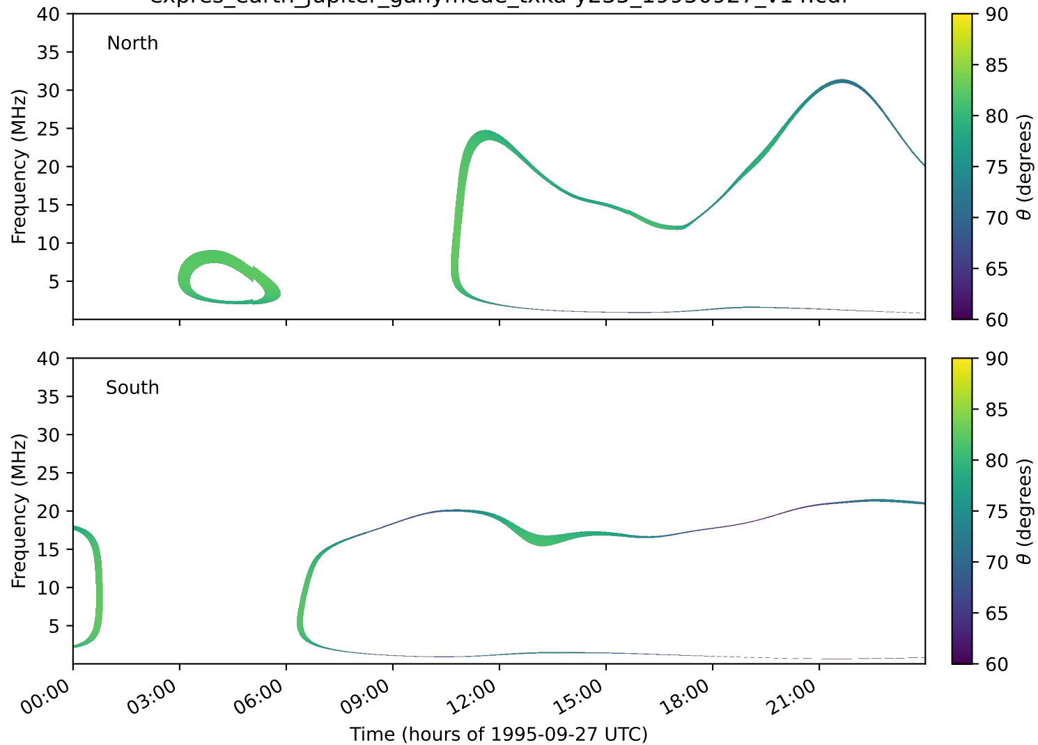
expres_earth_jupiter_ganymede_txka-y235_19950927_v14.cdf
