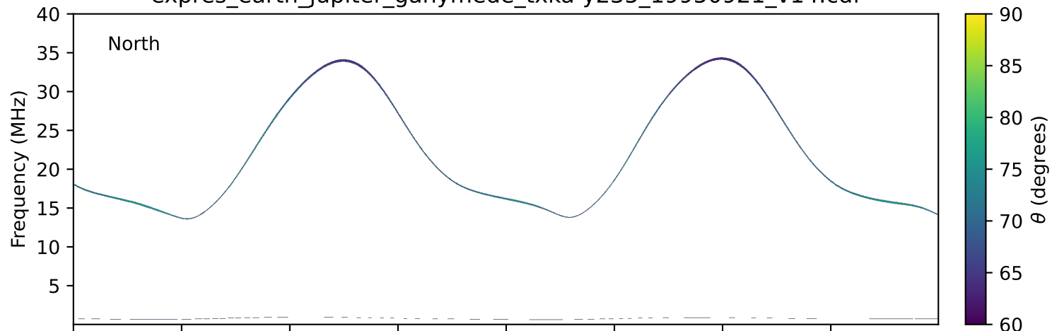
expres_earth_jupiter_ganymede_txka-y235_19950921_v14.cdf
