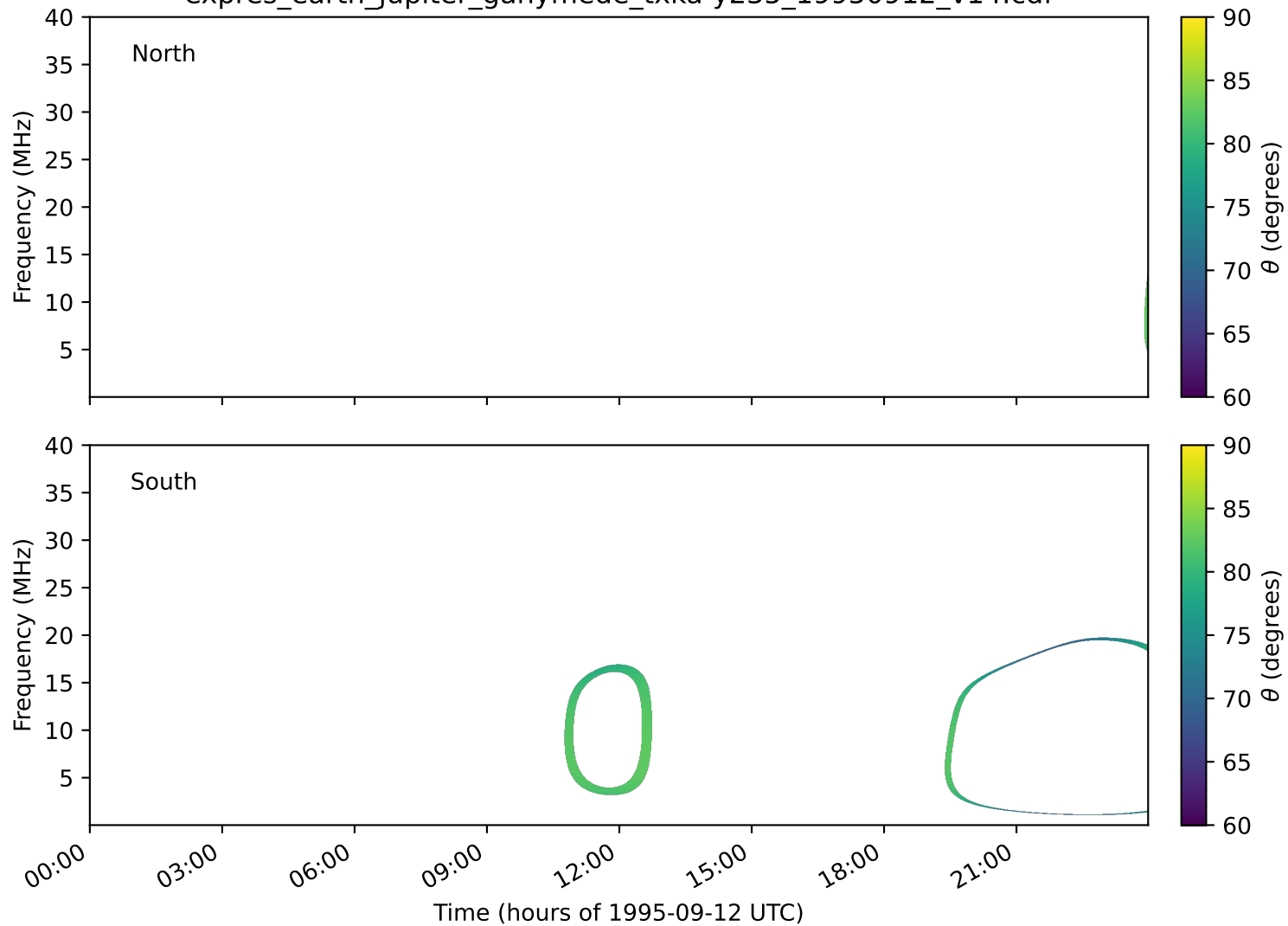
expres_earth_jupiter_ganymede_txka-y235_19950912_v14.cdf
