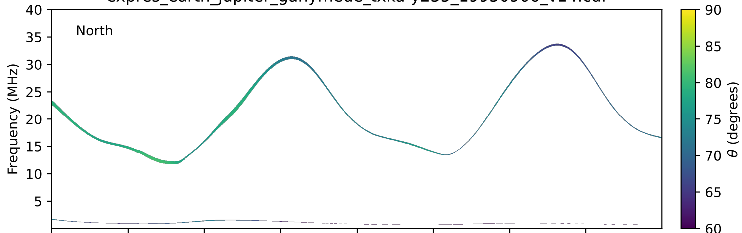
expres_earth_jupiter_ganymede_txka-y235_19950906_v14.cdf
