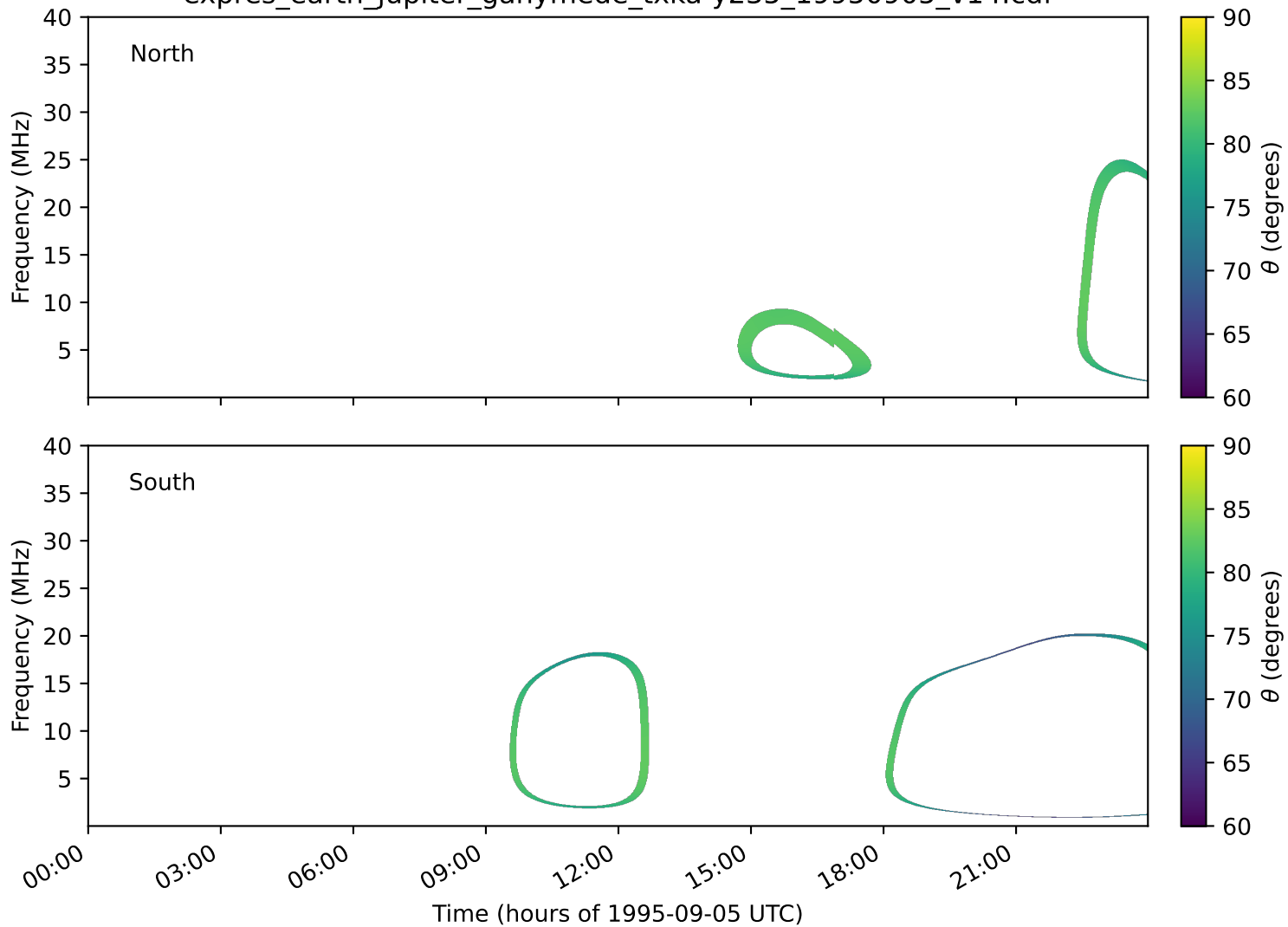
expres_earth_jupiter_ganymede_txka-y235_19950905_v14.cdf
