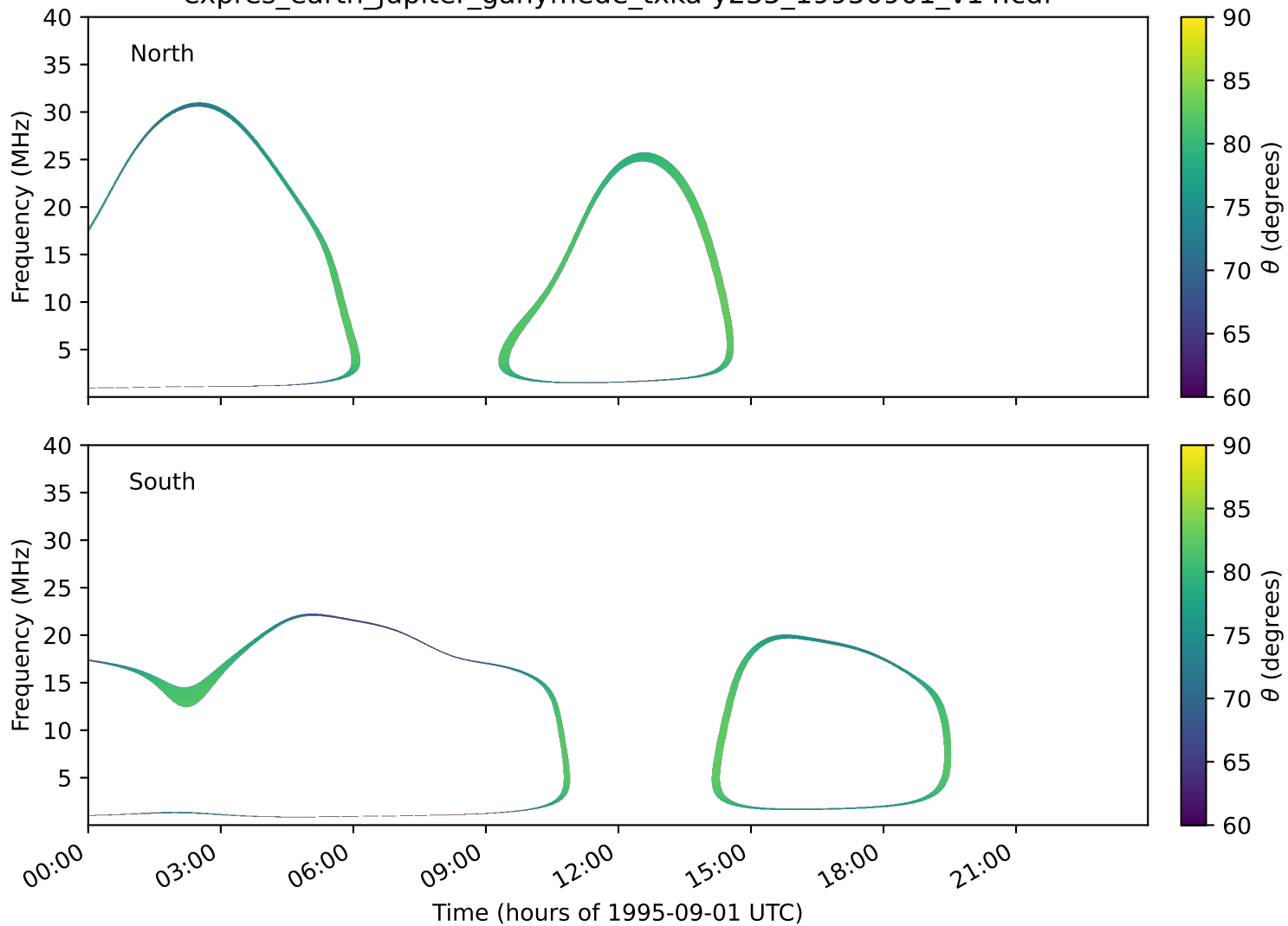
expres_earth_jupiter_ganymede_txka-y235_19950901_v14.cdf
