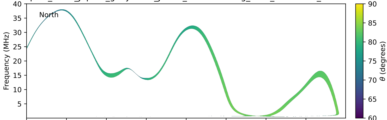
expres_earth_jupiter_ganymede_jrm33_lossc-wid1deg_3kev_19950901_v11.cdf
