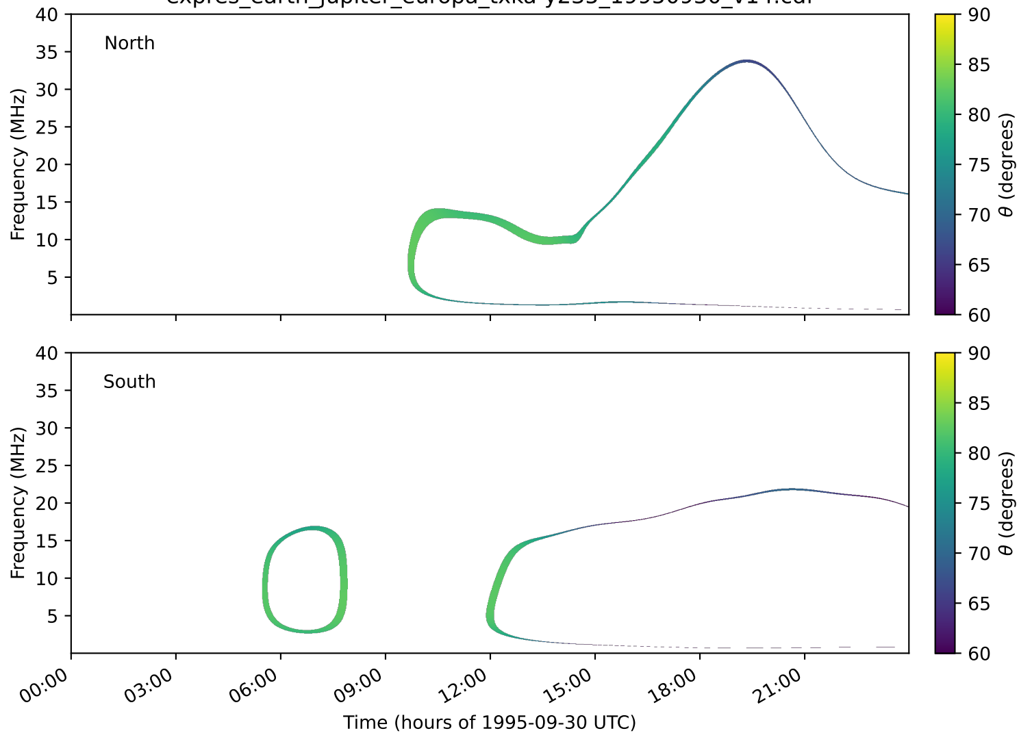
expres_earth_jupiter_europa_txka-y235_19950930_v14.cdf
