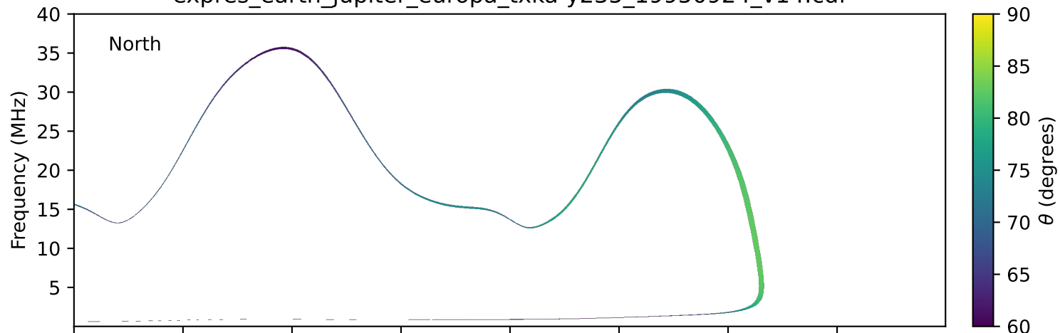
expres_earth_jupiter_europa_txka-y235_19950924_v14.cdf
