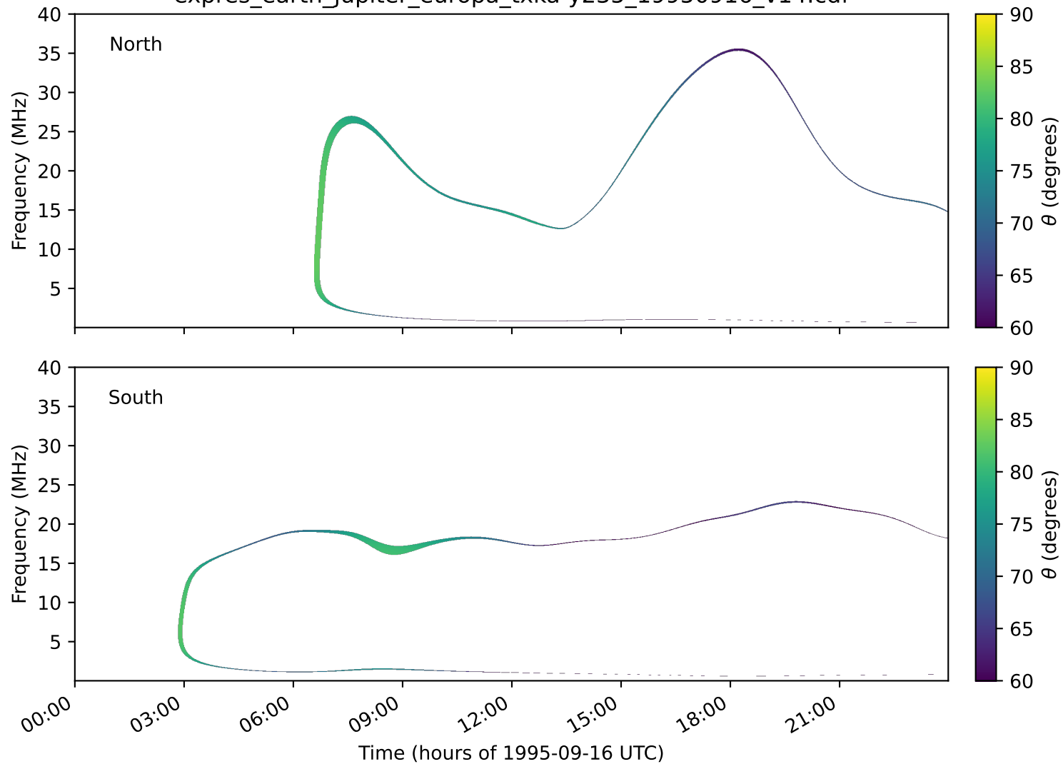
expres_earth_jupiter_europa_txka-y235_19950916_v14.cdf
