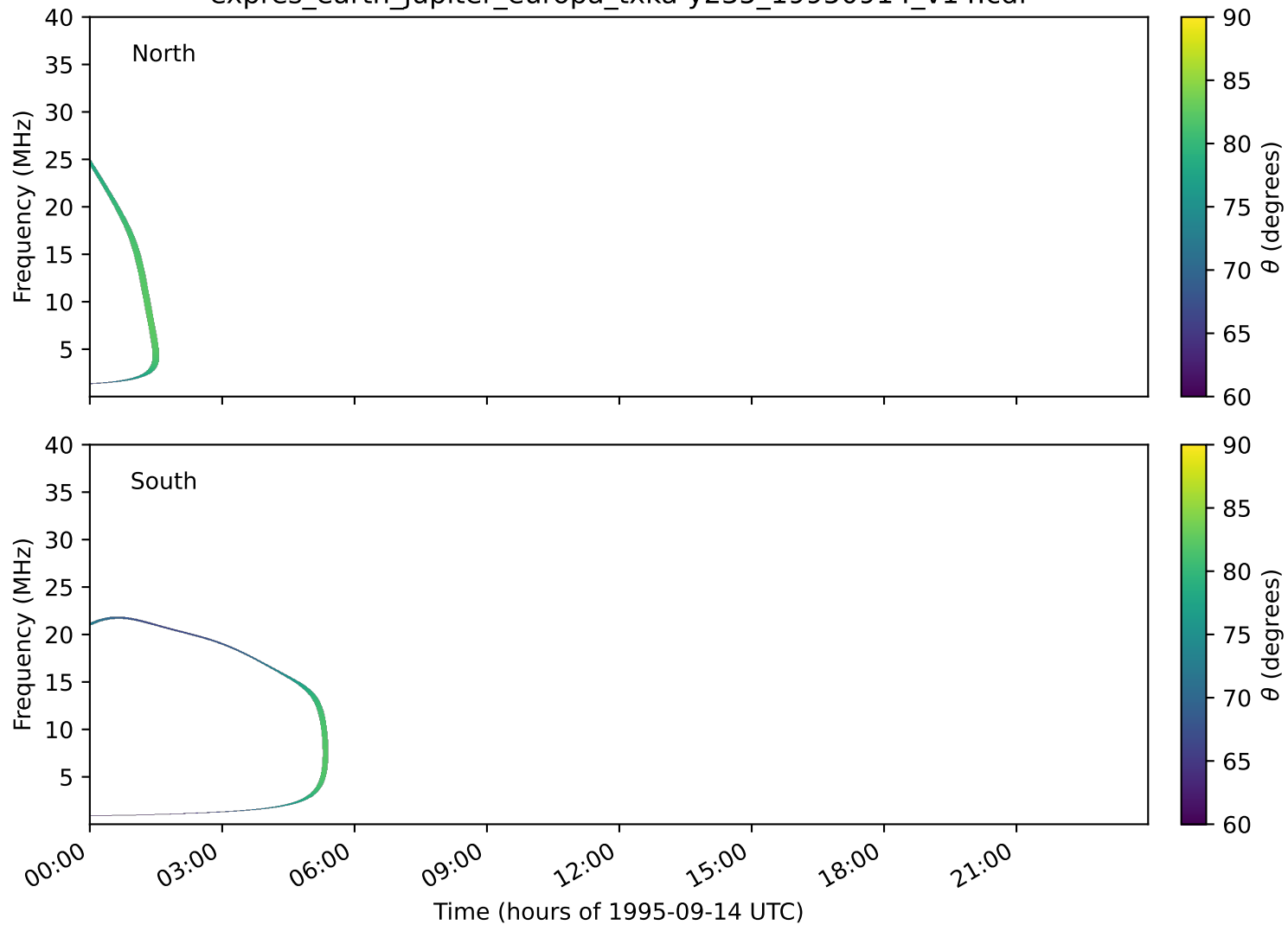
expres_earth_jupiter_europa_txka-y235_19950914_v14.cdf
