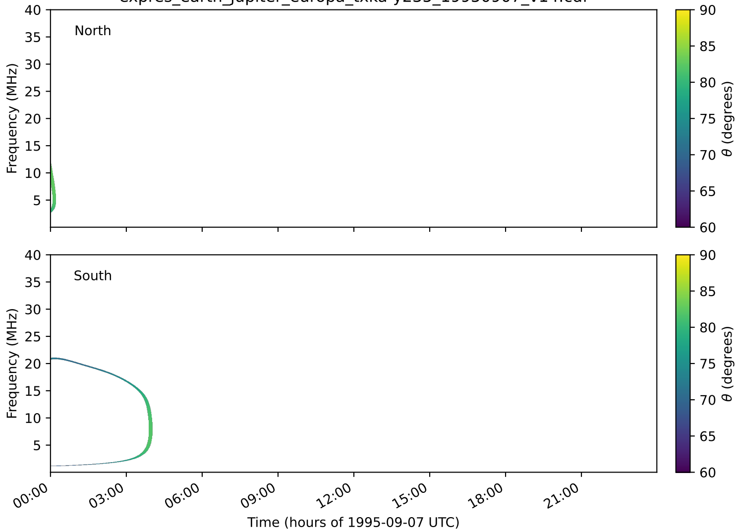
expres_earth_jupiter_europa_txka-y235_19950907_v14.cdf
