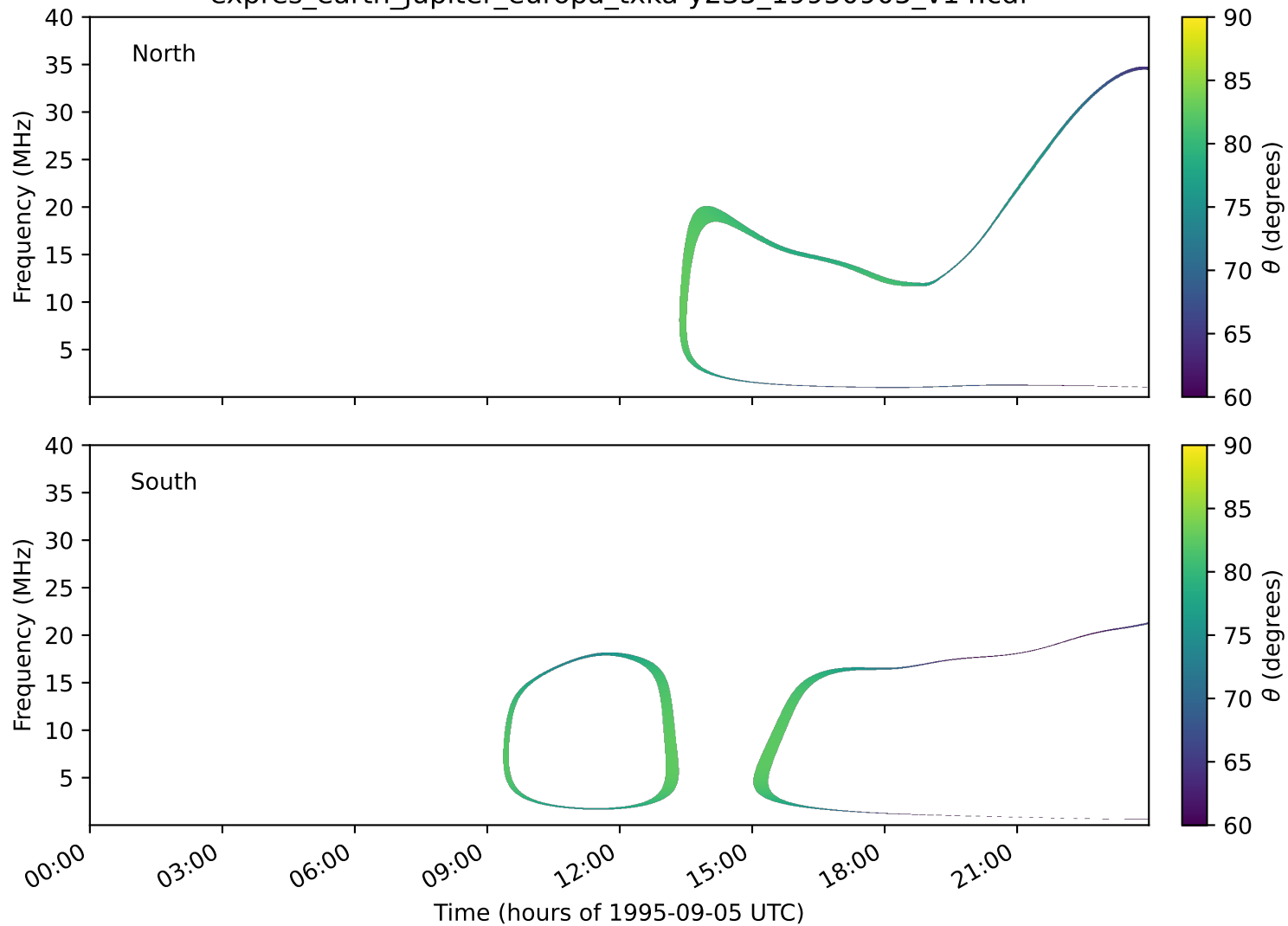
expres_earth_jupiter_europa_txka-y235_19950905_v14.cdf
