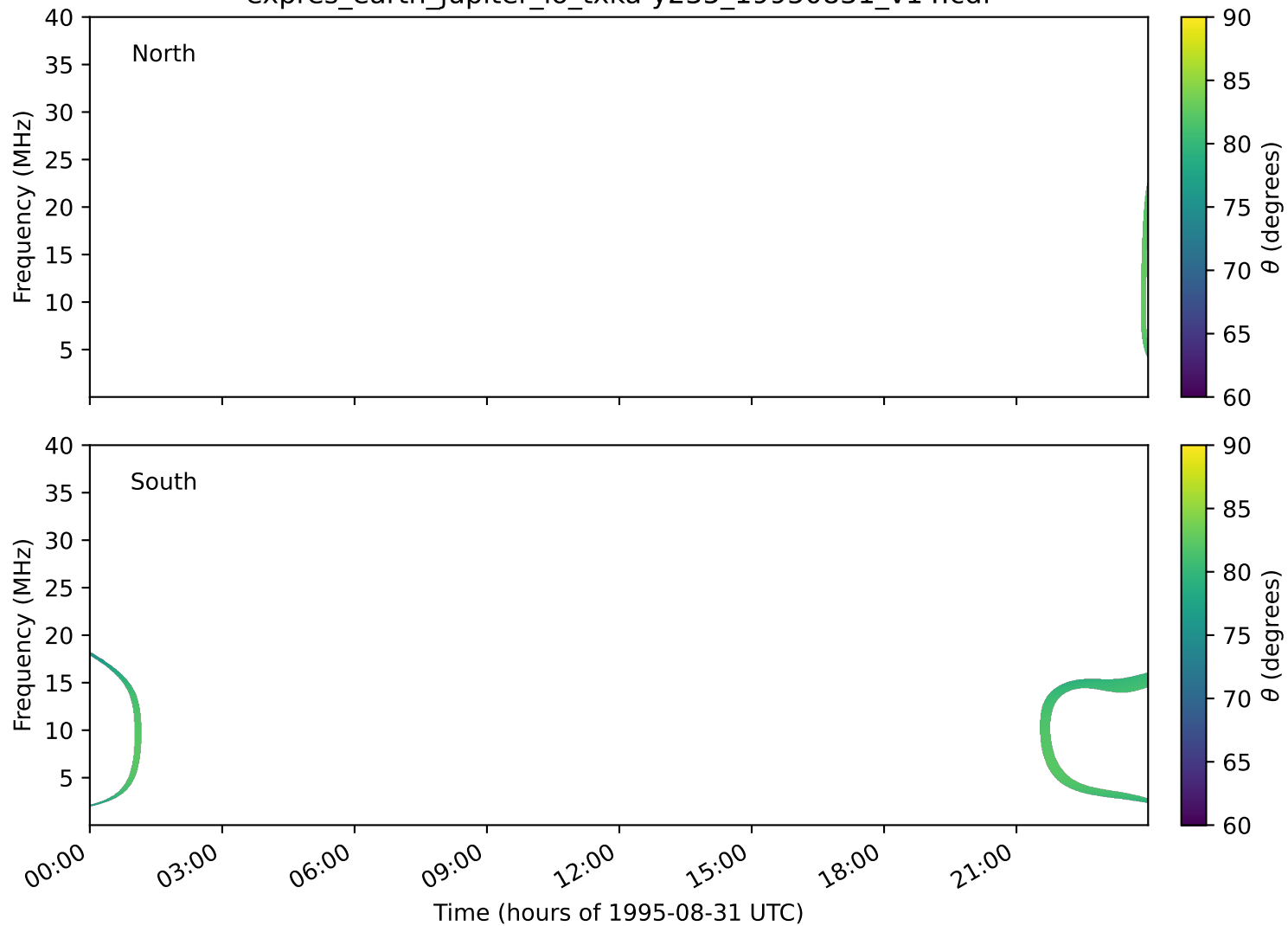
expres_earth_jupiter_io_txka-y235_19950831_v14.cdf
