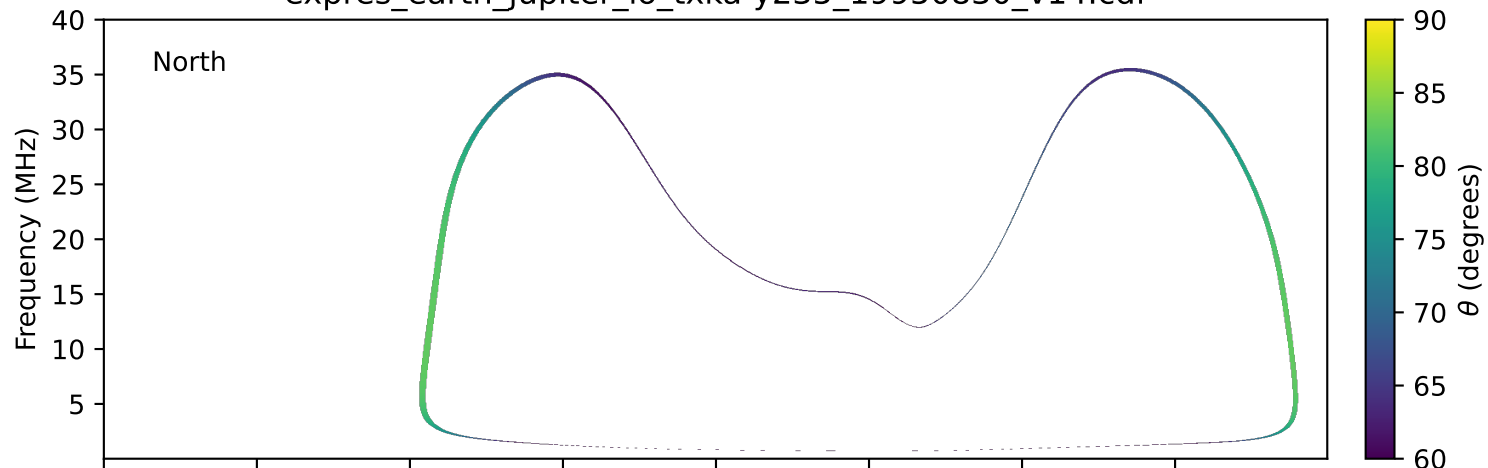
expres_earth_jupiter_io_txka-y235_19950830_v14.cdf
