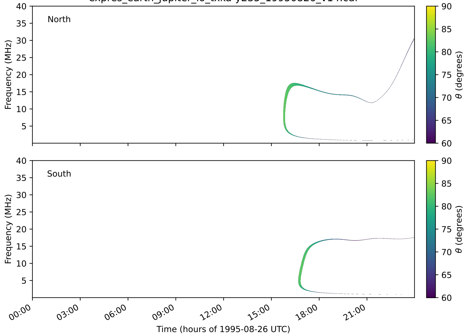
expres_earth_jupiter_io_txka-y235_19950826_v14.cdf
